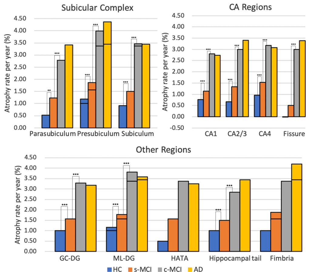
FIGURE 2 The atrophy rate of the hippocampal subfield volume ratio in each group. The black line indicates the atrophy rate of the whole hippocampus in the respective group. * indicates corrected p -values for the group comparisons. **, corrected p < .05 ; ***, corrected p < .01
